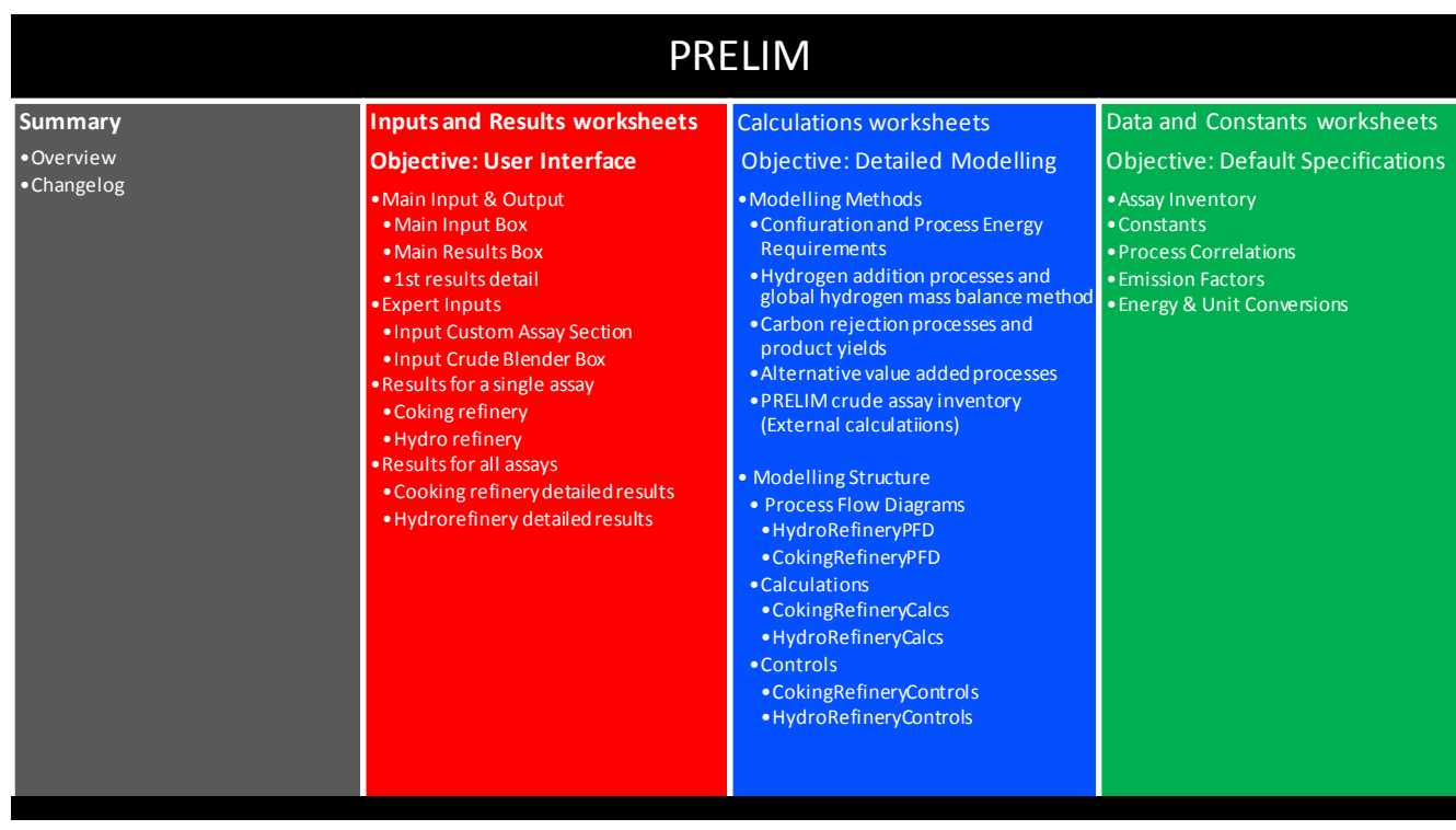
Figure 1 Overview of PRELIM software system organization.
