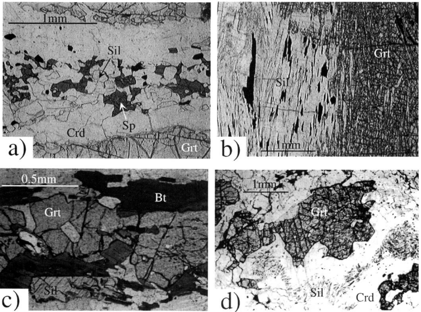
FIG. 4. Photomicrographs of granulite-facies mineral assemblages. Those shown in Figures 4a and 4b contain the assemblage Grt + Crd + Spl + Qtz + Sil + Kfs. a. Layer with the assemblage Sil + Crd + Spl sandwiched between two elongate grains of garnet. b. Strongly lineated sillimanite. c. The mineral assemblage Grt + Crd + Spl + Qtz + Sil + Kfs + Bt. Note the elongate shape of the garnet, which is characteristic of the metapelitic rocks in this area. This garnet also contains an inclusion of spinel. d. Adjacent grains of garnet and cordierite, with inclusions of sillimanite in both. Note the sillimanite-free rim around the cordierite, a common feature in many of the samples from this area.
