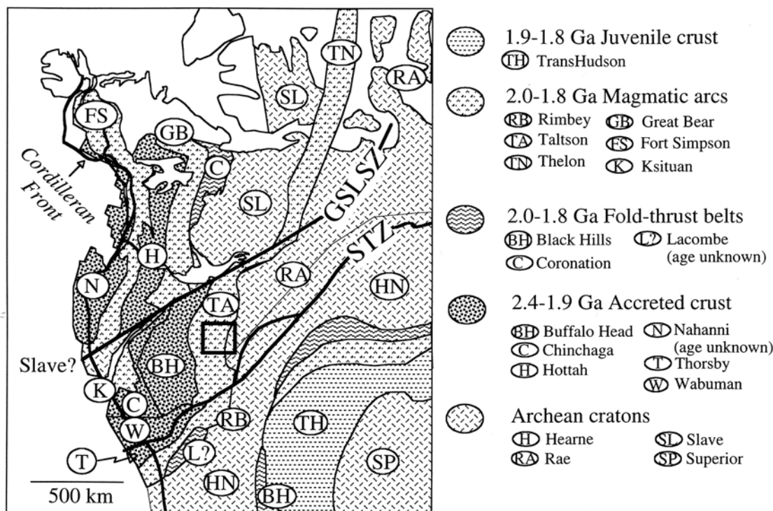
FIG. 1. Generalized geological map of western Laurentia, after Hoffman (1988) and Ross et al. (1991). The map area corresponds to the square. GSLSZ and STZ designate the Great Slave Lake Shear Zone and the Snowbird Tectonic Zone, respectively.
