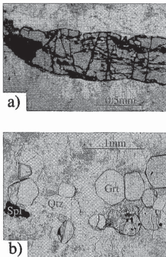
FIG. 6. Photomicrographs of garnet found in leucosomes. a. Elongate grain of garnet with inclusions of sillimanite and spinel. The texture suggests that this is relict garnet. b. Inclusion-free, euhedral grain of garnet, inferred to have been produced by the melting reaction.
