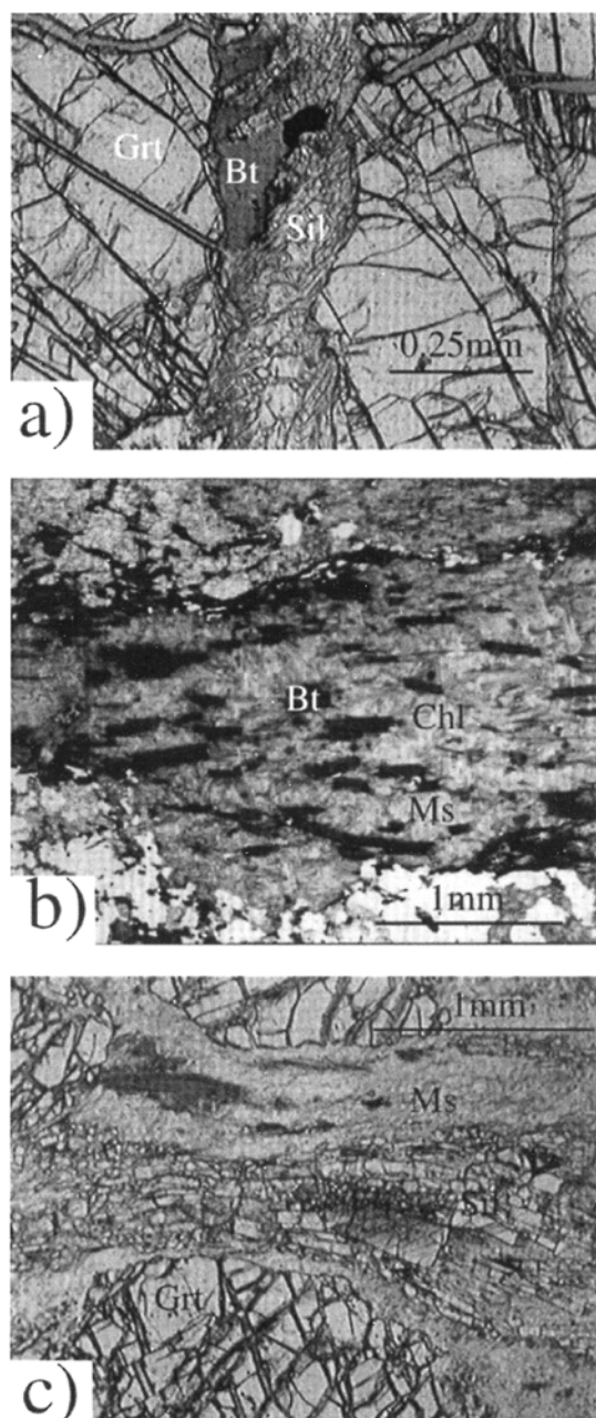
FIG. 8. Photomicrographs illustrating the overprinting of granulite-facies mylonites by lower-grade assemblages. a. Secondary biotite and sillimanite growing in the fracture of a deformed grain of garnet. b. The replacement of cordierite by biotite and chlorite. c. Fine-grained muscovite replacing K-feldspar.
