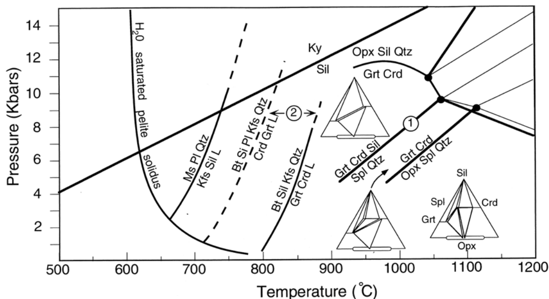
FIG. 5. Simplified phase diagram showing the experimentally determined reactions pertinent to the observed assemblages of minerals. \text{Ms} + \text{Pl} + \text{Qtz} = \text{Kfs} + \text{Sil} + \text{L} from Peto (1976). \text{Bt} + \text{Sil} + \text{Kfs} + \text{Qtz} = \text{Crd} + \text{Grt} + \text{L} (plagioclase-absent) from Carrington & Harley (1995). The position of the reaction \text{Bt} + \text{Sil} + \text{Pl} + \text{Kfs} + \text{Qtz} = \text{Crd} + \text{Grt} + \text{L} (plagioclase-bearing) is located approximately using data in Le Breton & Thompson (1988) and Vielzeuf & Holloway (1988), with slope parallel to the curve of Carrington & Harley (1995). The highest-grade Bt-absent reactions (system FMAS) are taken from Harley (1989).
