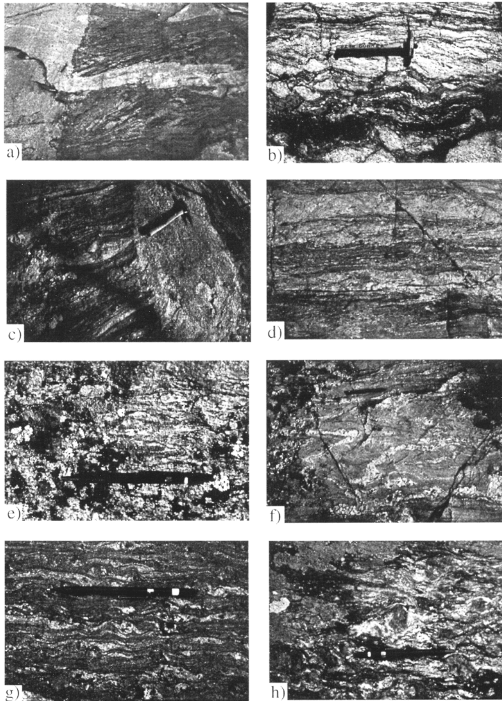
FIG. 3. Field photographs of metasedimentary rocks. a. A block of restitic paragneiss in Slave granite from Pelican Rapids along the Smith River. b. An outcrop along the shore of Andrew Lake showing metasedimentary schlieren deformed along with the enveloping granite. c. Well-foliated paragneiss cross-cut by a late dike of granite. d. Mylonitic paragneiss and granite. e. Elongate grains of garnet in the foliation plane. f. Garnet-bearing leucosomes in high-grade paragneiss. g and h. Deformed leucosome with asymmetrical tails.
