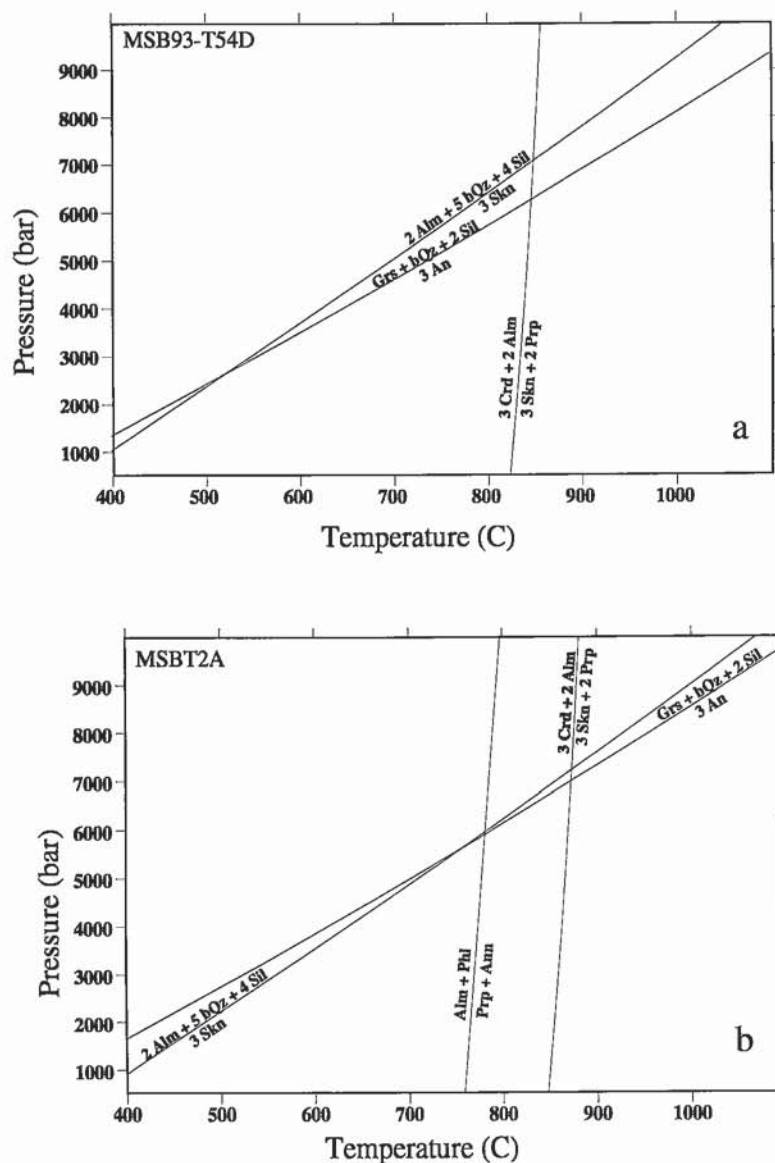
FIG. 7. a. Phase diagram illustrating the position of the calculated equilibria for sample MSB93-T54D, which contains the assemblage Grt + Sil + Spl + Crd + Pl + Qtz. The number of independent equilibria for this assemblage equals 3. b. Phase diagram illustrating the positions of the calculated equilibria for sample MSBT2A, which contains the above assemblage plus biotite. There are four independent equilibria for this assemblage. Skn stands for sekaninaite, the Fe end-member of cordierite.
