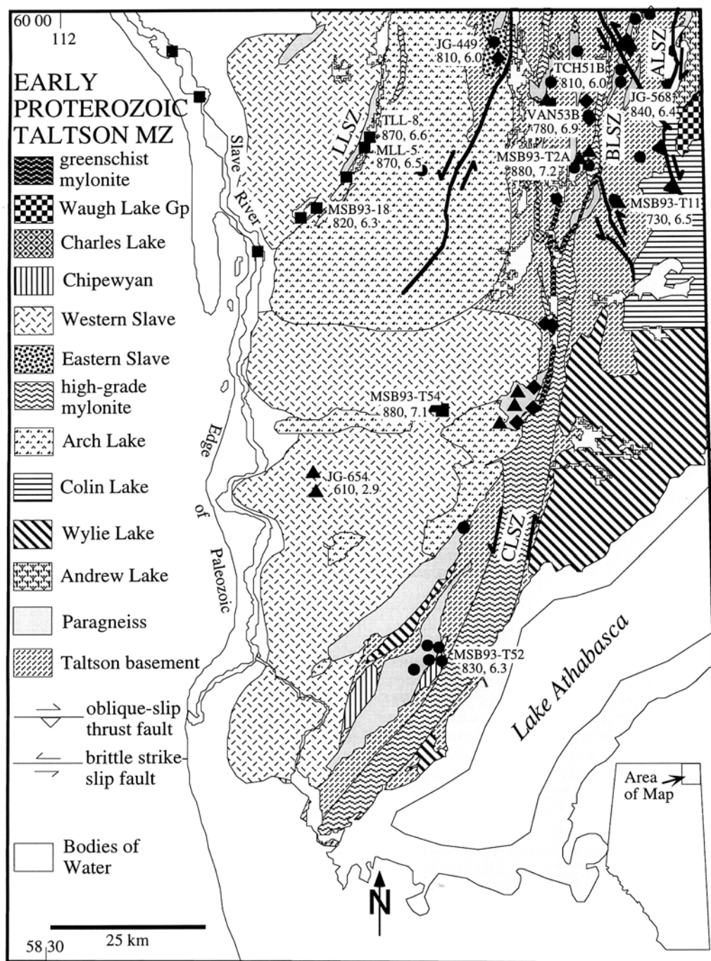
FIG. 2. Generalized geological map of the southern Taltson Magmatic Zone, after McDonough et al. (1997), and assemblage map showing the distribution of assemblages of high-grade metamorphic minerals. LLSZ, CLSZ, BLSZ, and ALSZ designate the Leland Lake, Charles Lake, Bayonet Lake and Andrew Lake shear zones, respectively. Mineral assemblages as follows: squares: Spl + Qtz + Grt + Crd + Kfs + Sil; triangles: Spl + Qtz + Bt + Grt + Crd + Kfs + Sil; circles: Grt + Bt + Crd + Kfs + Sil + Qtz, with Spl inclusions in Grt and Crd; diamonds: Grt + Bt + Crd + Kfs + Sil + Qtz. P-T estimates are taken from Table 6 and are discussed in the text. The temperature estimates are based on the Grt-Crd Fe-Mg exchange equilibrium.
