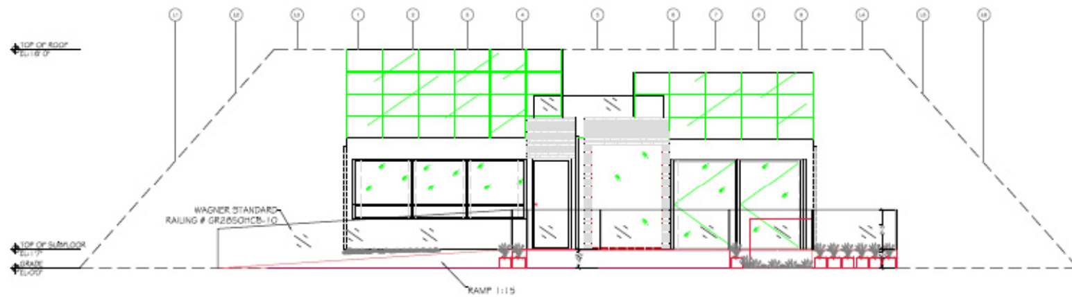
2 SOUTH SOLAR ENVELOPE L-201 1" = 1'0"
