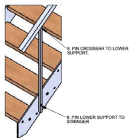
DETAIL C SCALE 1 : 10
