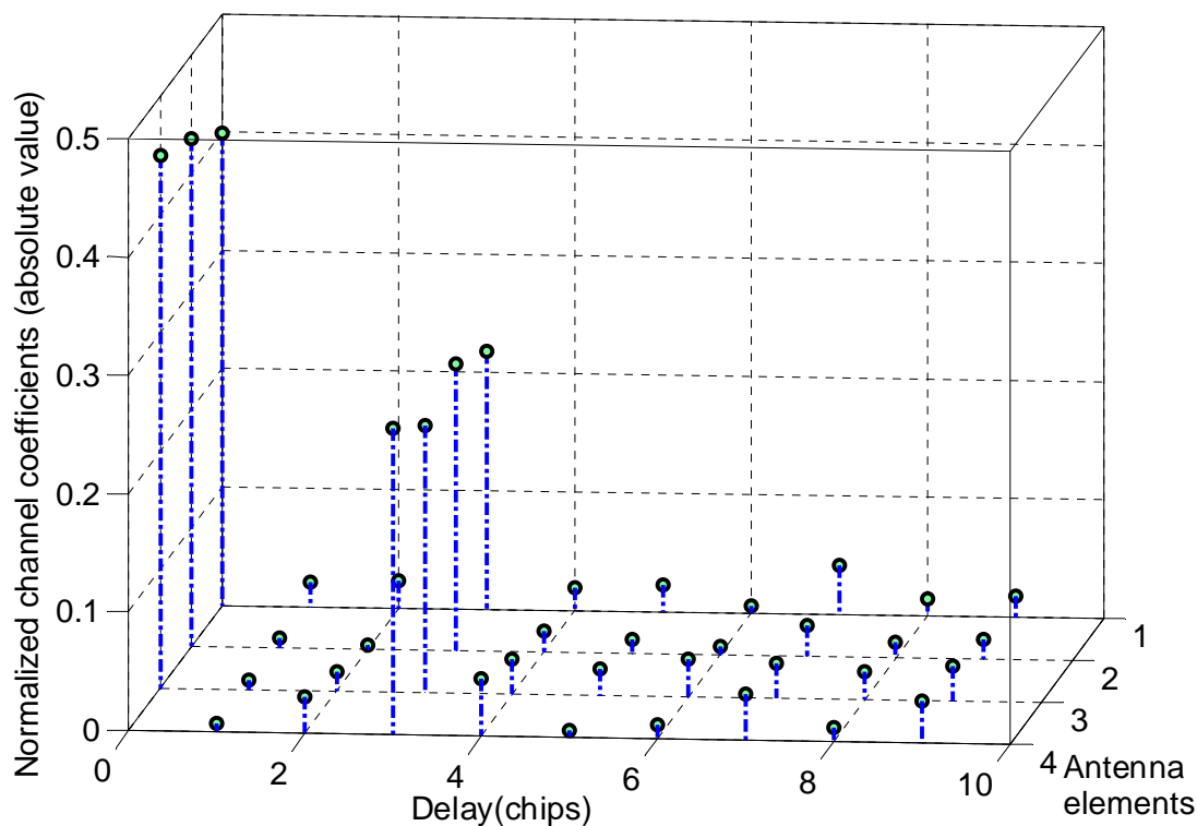
Figure 6-3: The absolute values of the estimated channel coefficients for the LOS and one multipath component of the spoofing signal
