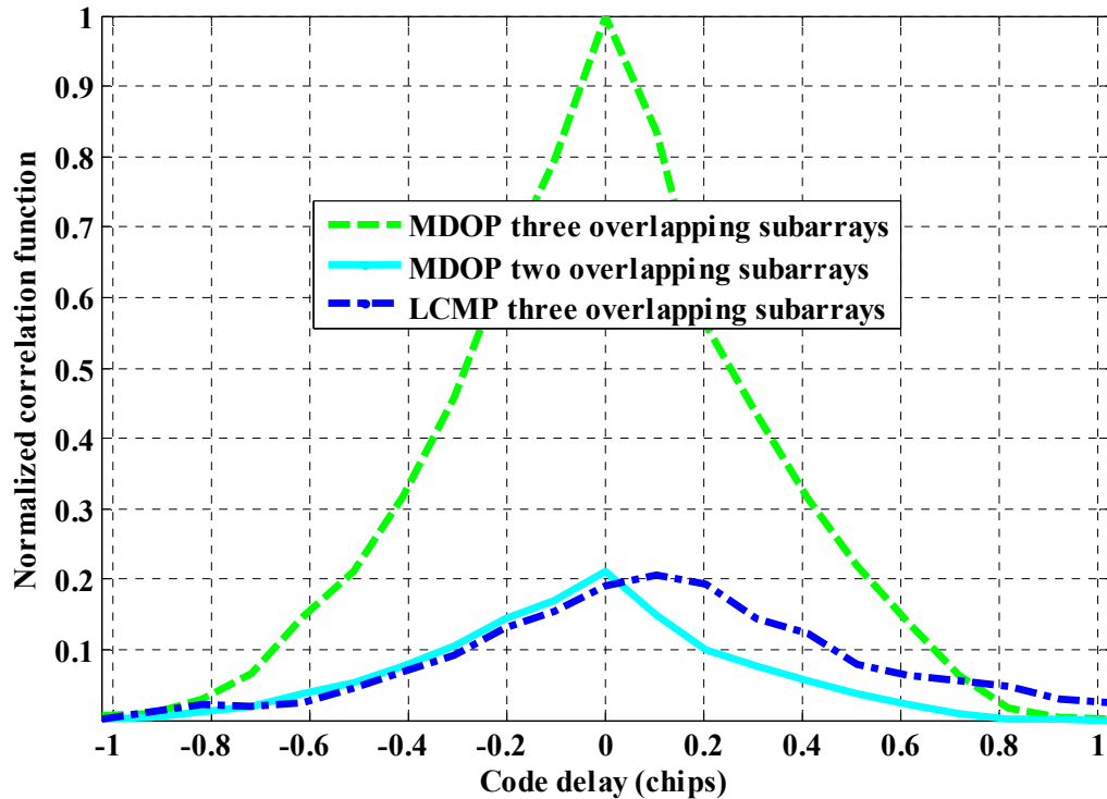
Figure 3-5: Correlation functions for the MDOP method with three overlapping subarrays, the MDOP method with two overlapping subarrays and the LCMP beamformer with three overlapping subarrays
