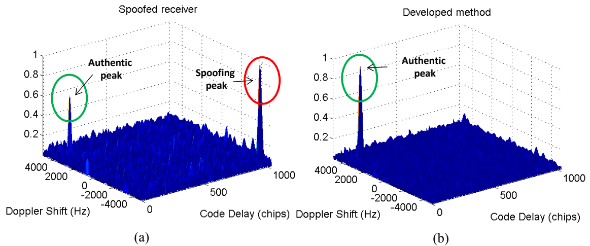
Figure 6-5: Normalized CAFs (a) before spoofing mitigation (b) after spoofing mitigation
